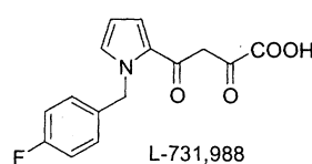
Fig. 1. Activity (IC 50 , in μM) of diketo acid inhibitors. PIC, preintegration complex.
