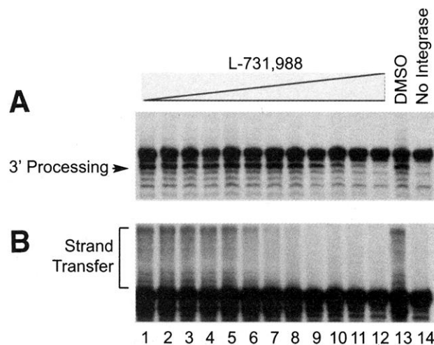
Fig. 3. Inhibition of 3' processing and strand transfer by L-731,988. (A) Integrase 3' processing and (B) strand transfer activities are shown. HIV-1 HXB-2 integrase (1 μM) was incubated with 50 nM of a 32 P-labeled oligonucleotide representing the last 20 nucleotides of the HIV-1 U5 end. Reactions included varying levels of L-731,988 (threefold dilutions from 100 μM, lane 12, to 5 × 10 -4 μM, lane 1). Reactions were performed for 1 hour at 37°C and analyzed as described (18).
